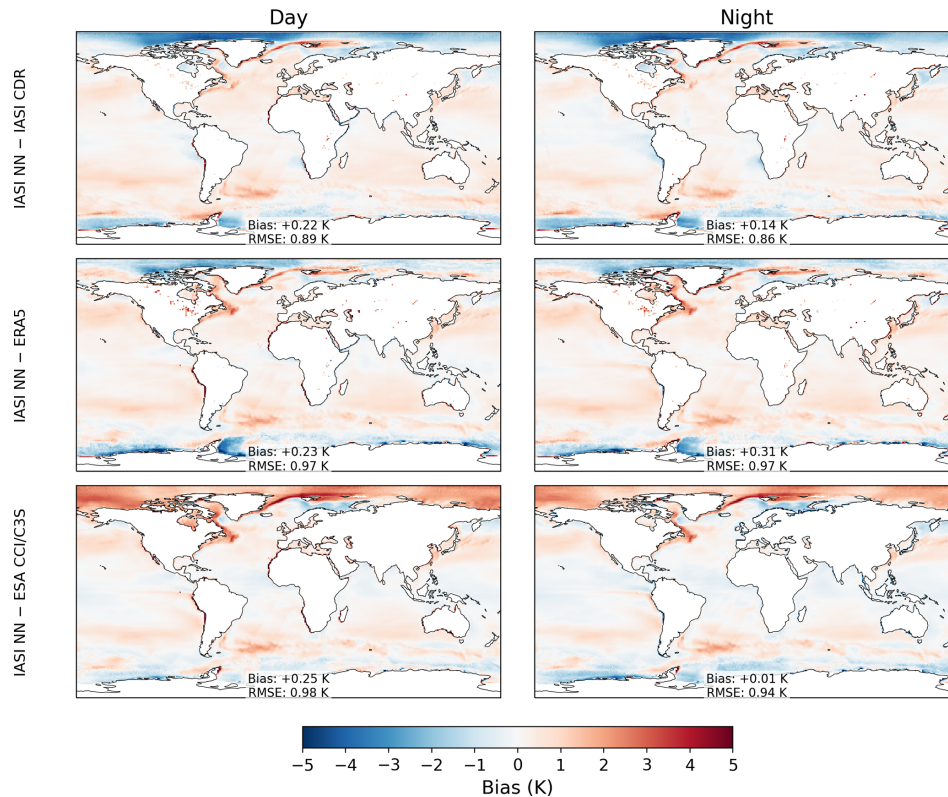
Figure 5. Spatial bias of IASI-NN ocean skin temperature relative to IASI-CDR, ERA5, and the ESA CCI/C3S SST analysis. Maps show daytime (left column) and nighttime (right column) biases, computed as the time mean of the monthly-mean differences over the datasets' common period (2008–2022). The ESA CCI/C3S product is a gap-filled, all-sky, with no day/night separation, so the same daily field is differenced against both the daytime and nighttime IASI-NN fields; IASI and ERA5 are restricted to clear-sky scenes. All datasets were regridded to a common 1^\circ \times 1^\circ grid and land points were masked using the ERA5 land–sea mask. Sea-ice-covered grid cells are classified as ocean by this mask and are therefore included. Global mean bias and RMSE, area-weighted by the cosine of latitude, are indicated in each panel.
