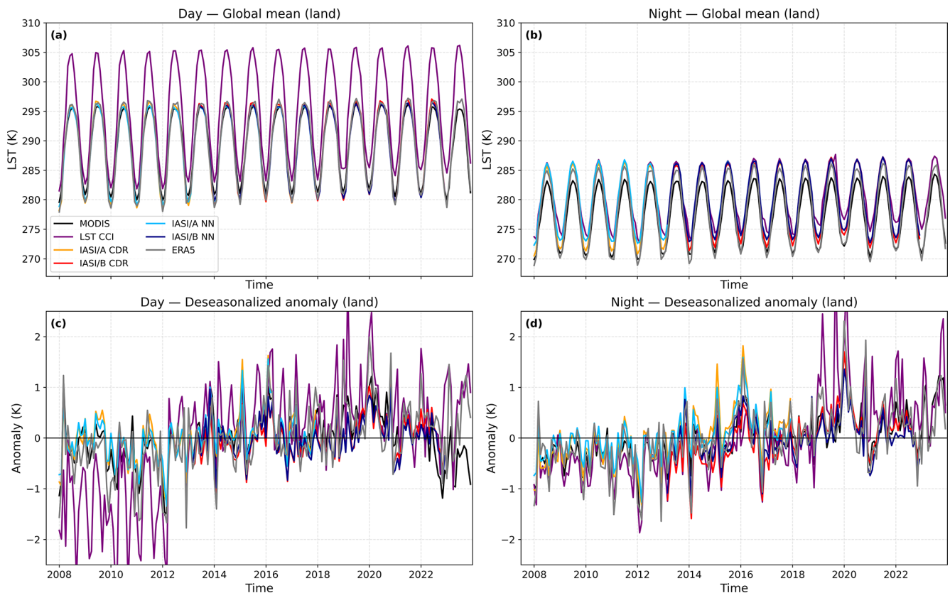
Figure 1. Global mean land surface temperature (LST, a , b ) and deseasonalised anomalies ( c , d ) for daytime ( a , c ) and nighttime ( b , d ). IASI Metop-A and Metop-B observations (IASI-A/B) are shown separately for the CDR and NN products. Global means are computed using cosine-latitude weighting.
