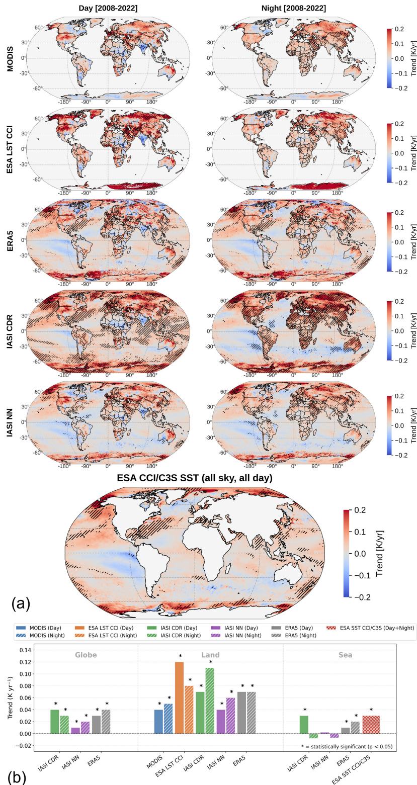
Figure 6. (a) Spatial trends [K yr -1 ] during day (left column) and night (right column) for MODIS, ESACCI LST, ERA5, IASI-CDR, IASI-NN, and ESA CCI/C3S SST (all sky, all day) over the period January 2008–December 2022. Stipples correspond to regions where trends are significant according to the standard Mann-Kendall test ( p -value < 0.05 ). (b) Global (T skin ), sea (SST), land (LST) trends (K yr -1 ) from MODIS, ESA CCI LST, IASI-CDR, IASI-NN, ERA5, and ESA CCI/C3S SST over the period [January 2008–December 2022]. Trends are computed with the Theil–Sen estimator on annual latitude-weighted and deseasonalised averages. Significant trends are marked with an Asterisk (*) above the bars.
