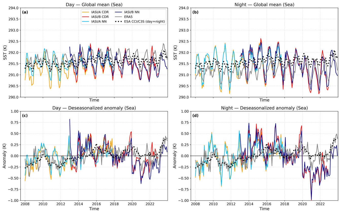
Figure 4. Upper panels: SST global mean during the day (a) and the night (b) for ERA5, IASI-CDR and IASI-NN, and ERA5 CCI and C3S SST all-sky product which is shown in dotted black line. It is the same for the day and night panels as it is a combined product. IASI data are separated between Metop A and Metop B. Lower panels: the deseasonalized anomaly of SST for the different products, during the day (c) and night (d). Global means are computed using cosine-latitude weighting.
