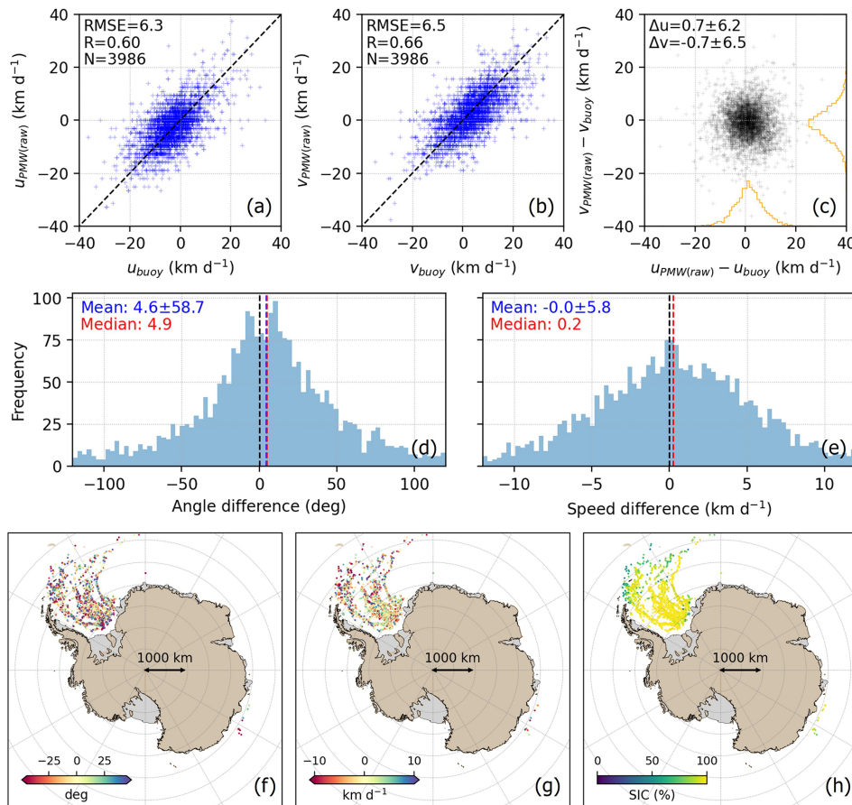
Figure 8. (a) Scatter plot between u -component sea ice drift from buoys and raw PMW feature tracking (without interpolation; PMW_{raw} ), (b) scatter plot between v -component sea ice drift from buoys and PMW_{raw} . (c) Error distribution of the u and v sea ice drift components. (d) Distribution of angle difference and (e) speed difference between PMW_{raw} and buoy sea ice velocities. Location of buoys visualized by (f) angle difference, (g) speed difference, and (h) sea ice concentration.
