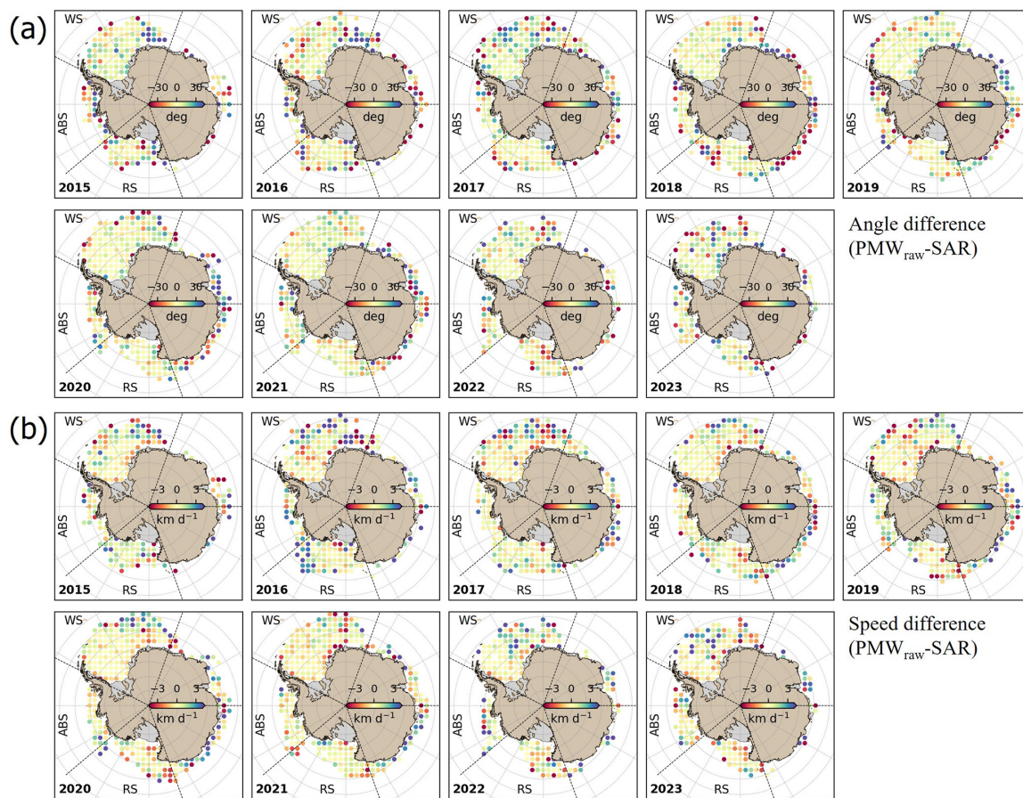
Figure 11. (a) Map of the angle difference between \text{PMW}_{\text{raw}} and SAR sea ice drift from 2015 to 2023. Positive angle difference (bluish color) indicates the \text{PMW}_{\text{raw}} ice drift vector is clockwise rotated to the SAR ice drift vector, and negative angle difference (reddish color) means the anti-clockwise rotation of the \text{PMW}_{\text{raw}} drift vector relative to the SAR ice drift vector. (b) Map of speed difference between \text{PMW}_{\text{raw}} and SAR sea ice drift from 2015 to 2023.
