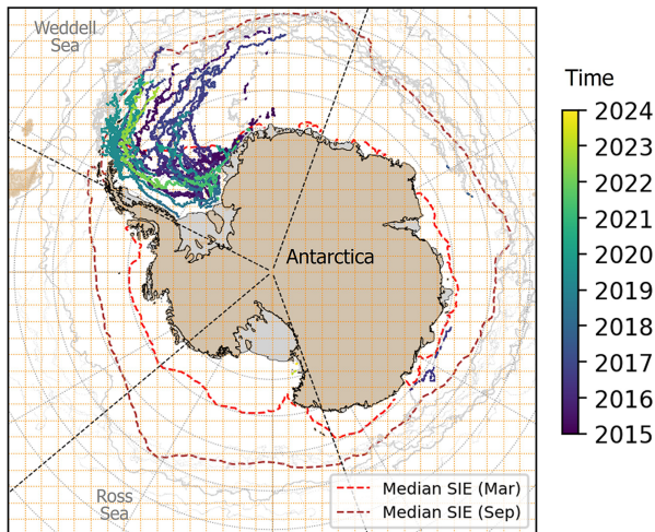
Figure 2. Distribution of Antarctic drifting buoys from 2015 to 2023. The buoys inside sea ice cover (SIC > 15 %) are colored by the times of the buoy locations, whereas the buoys outside sea ice cover are displayed in gray points. The red dashed line indicates the median March sea ice extent (SIE) in 1981–2010, and the brown dashed line indicates the median September SIE in 1981–2010. While most of the buoys are deployed in the Weddell Sea, these buoys rarely pass through the sea ice area in other regions. Orange dashed lines show the 250 km \times 250 km super-grid for Sentinel-1 data collection.
