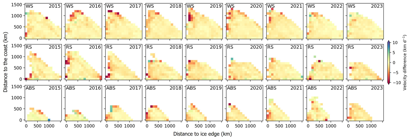
Figure 12. Speed difference between PMW and SAR sea ice drift by the distance to ice edge ( x -axis) and coast ( y -axis) for Weddell Sea (WS), Ross Sea (RS), and Amundsen-Bellinghousen Seas (ABS) from 2015 to 2023.
