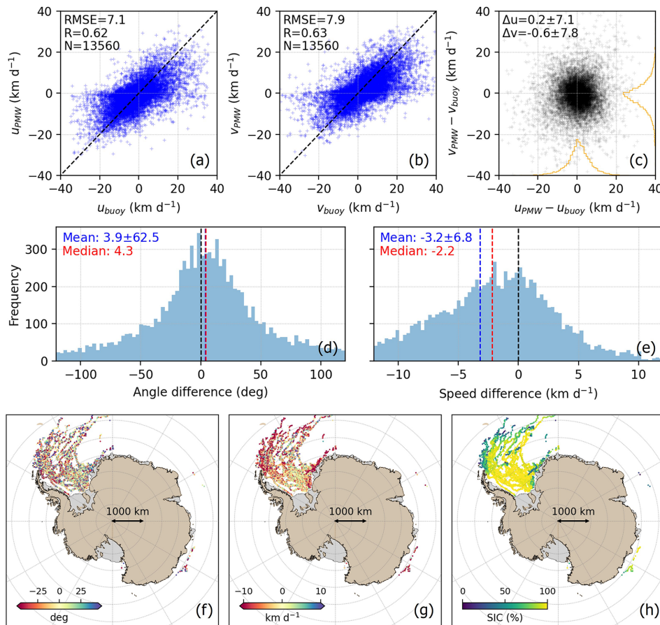
Figure 4. (a) Scatter plot between u -component sea ice drift from buoys and PMW, (b) scatter plot between v -component sea ice drift from buoys and PMW. (c) Error distribution of the u and v sea ice drift components. (d) Distribution of angle difference and (e) speed difference between PMW and buoy sea ice velocities. Location of buoys visualized by (f) angle difference, (g) speed difference, and (h) sea ice concentration.
