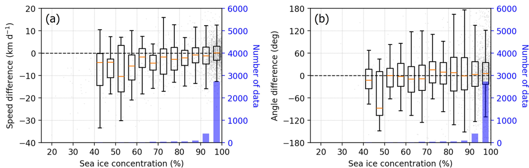
Figure 9. (a) Speed difference between raw PMW (without interpolation; PMW_{raw} ) and buoy sea ice drift by sea ice concentration. (b) Angle difference between PMW_{raw} and buoy sea ice drift by sea ice concentration.
