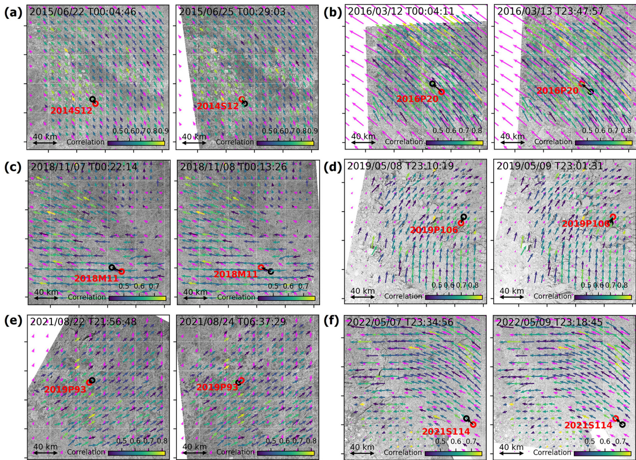
Figure 1. Derivation of sea ice drift from SAR images nearby (a) buoy 2014S12 from 22 to 25 June 2015, (b) buoy 2016P20 from 12 to 13 March 2016, (c) buoy 2018M11 from 7 to 8 November 2018, (d) buoy 2019P106 from 8 to 9 May 2019, (e) buoy 2019P93 from 22 to 24 August 2021, and (f) buoy 2021S114 from 7 to 9 May 2022. Colored arrows indicate SAR-derived sea ice drift, with colors representing the correlation of feature tracking (see bottom-right color bar). Magenta arrows indicate PMW sea ice drift, and black arrows indicate the movements of buoys between the SAR acquisition times; red circles denote the location of the buoy at each image, and buoy IDs are annotated in red. The lengths of the vectors correspond to the actual sea ice displacement.
