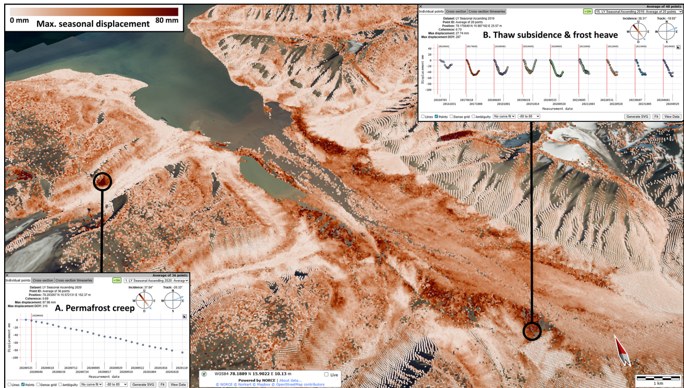
Figure 2. Example of seasonal InSAR Svalbard results in the Longyearbyen (LY) study area. The map displays the maximum seasonal displacement expressed in mm (here for 2020, using an ascending SAR geometry). (A) When analysing one SAR geometry and one season, the seasonal time series provide information on the short-term displacement pattern during the spring–fall snow-free period (here on a rock glacier). (B) When all seasons and geometries are viewed all together, the time series provide information about the magnitude and timing of the displacement patterns during multiple seasons (here cyclic subsidence–heave patterns in an ice-rich part of the Advent valley). The results are shown in the InSAR Svalbard WebGIS tool. Background: Svalbard Orthophoto (NPI, 2026).
