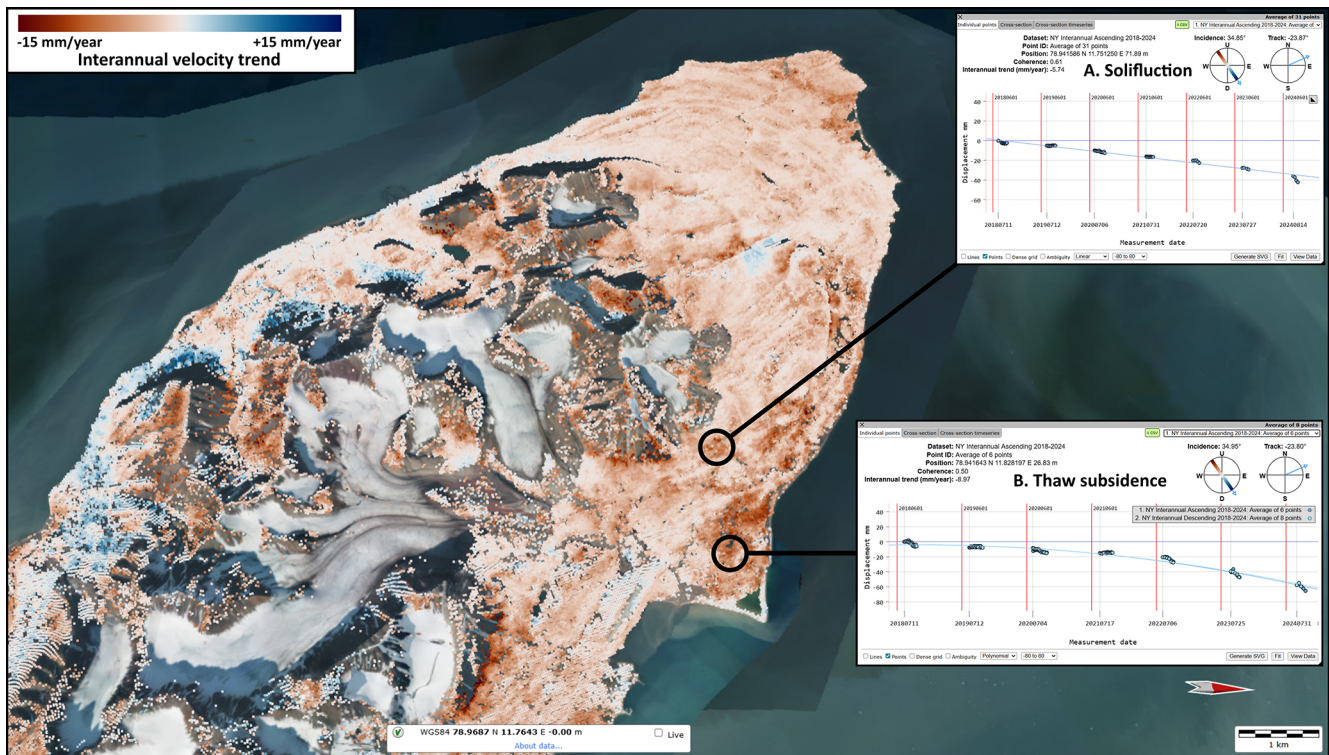
Figure 3. Example of interannual InSAR Svalbard results in the Ny-Ålesund (NY) study area. The map displays the mean annual velocity expressed in \text{mm yr}^{-1} (here for 2018–2024 using an ascending SAR geometry). (A) The interannual displacement time series provide information on long-term gradual displacements occurring on mountain slopes (here due to solifluction). (B) In flat terrain, the results provide information on interannual changes of surface levels (here accelerating thaw subsidence, likely due to top-of-permafrost ice melt). The results are shown in the InSAR Svalbard WebGIS tool. Background: Svalbard Orthophoto (NPI, 2026).
