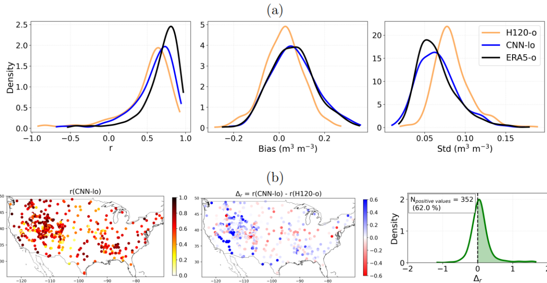
Figure 3. (a) Probability density functions (PDF) of temporal correlation ( r ), error bias (Bias, \text{m}^3 \text{m}^{-3} ), and standard deviation of error (SD, \text{m}^3 \text{m}^{-3} ) for ERA5-o, CNN-lo, and H120-o against in situ measurements at 568 sites across CONUS in 2019. (b) Maps showing (left) correlation of CNN-lo with in situ data and (middle) improvement in correlation with in situ data for CNN-lo relative to H120-o ( \Delta_r = r(\text{CNN-lo}) - r(\text{H120-o}) ). Blue (red) indicates improved (degraded) correlation. The PDF of this \Delta_r is also presented in the right panel.
