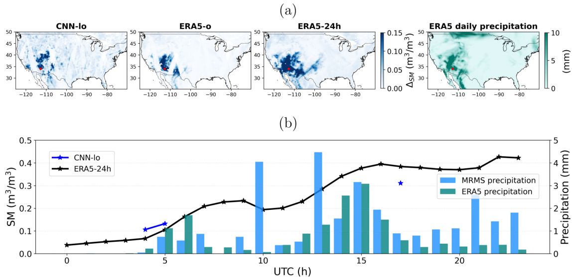
Figure 6. (a) Maps of daily SM amplitude ( \Delta_{SM} ) on 20 November 2019, derived from CNN-lo and ERA5-o. ERA5-24h (full 24 h amplitude) and daily accumulated precipitation are also shown for reference. (b) Hourly SM time series at [34^\circ \text{ N}, 112.75^\circ \text{ W}] (marked with a red dot in the maps), comparing CNN-lo retrievals to ERA5-24h. CNN-lo estimates correspond to three ASCAT overpasses: two ascending (04:00–05:00 UTC) and one descending (17:00 UTC). Precipitation data from both the independent MRMS gauge-corrected product and ERA5 are also presented.
