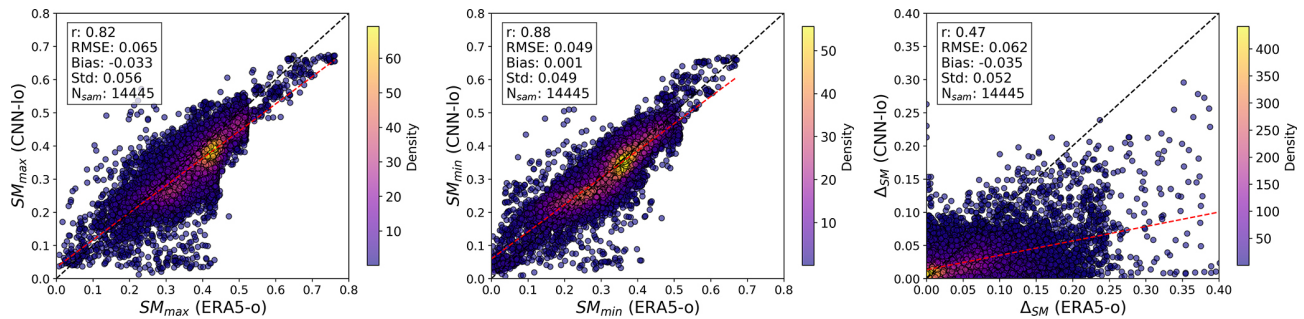
Figure 8. Scatter plots comparing CNN-lo and ERA5-o SM for days with isolated precipitation events ( p_t > 10 mm and p_{t-1} = 0 mm) in 2019. Panels show: (1) maximum SM value ( SM_{\max} ); (2) minimum SM value ( SM_{\min} ); and (3) the resulting diurnal SM amplitude ( \Delta SM = SM_{\max} - SM_{\min} ), all in \text{m}^3 \text{m}^{-3} . Each point represents one pixel-day. Statistical metrics include total correlation ( r ), root mean square error (RMSE, \text{m}^3 \text{m}^{-3} ), bias (Bias, \text{m}^3 \text{m}^{-3} ), standard deviation (SD, \text{m}^3 \text{m}^{-3} ), and number of samples ( N_{\text{samples}} ). The dashed black line represents the 1 : 1 line; the red dashed line is the linear regression fit. The colorbar indicates the local density of dots in the scatterplot.
