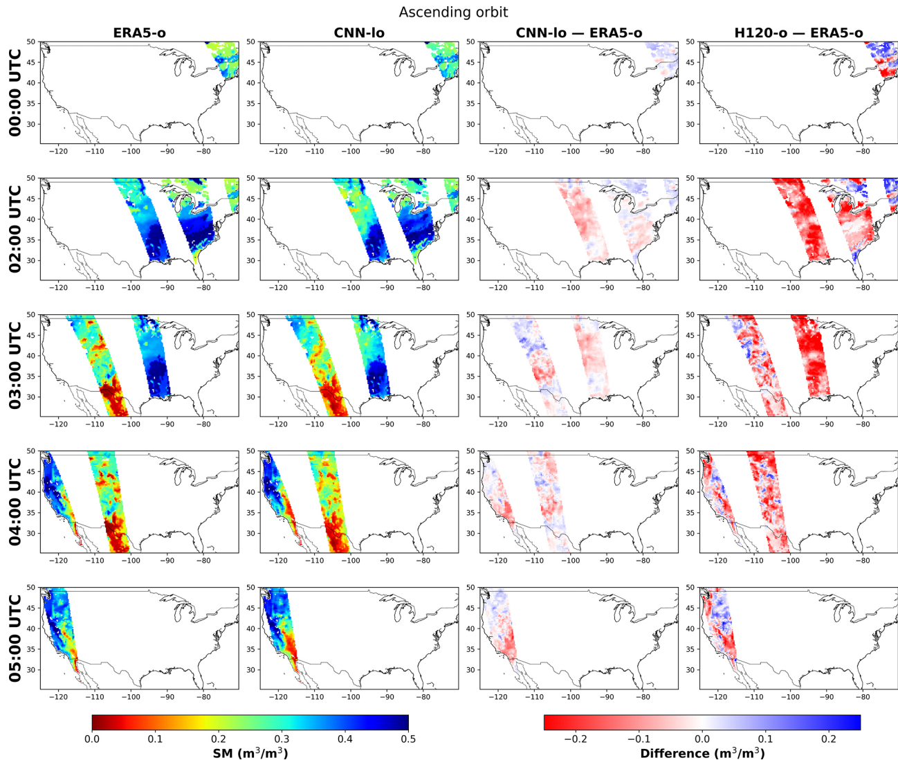
Figure 2. Hourly soil moisture (SM) estimates corresponding to five ascending ASCAT overpasses (00:00–05:00 UTC) on 20 January 2019. The first and second columns display SM values from ERA5-o and CNN-lo, respectively. The third column shows the SM differences between CNN-lo and ERA5-o, while the fourth column presents differences between H120-o and ERA5-o.
